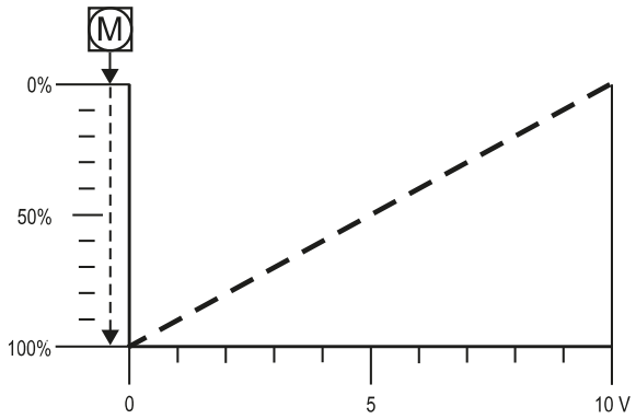
Figure 16: The dip switch 4 ON (Reversing Acting – RA) When the signal increases the actuator stem retracts.
