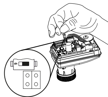
Figure 19: Stroke options
