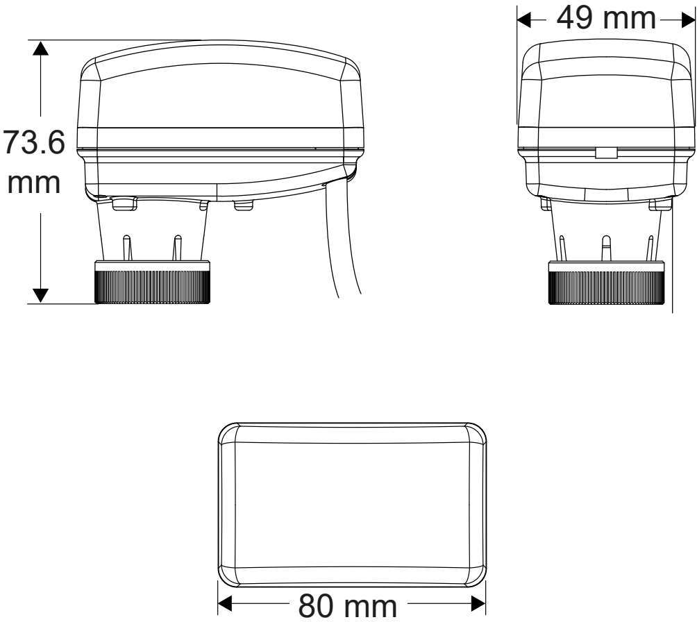
Figure 20: Actuator dimensions
